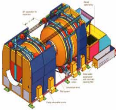
Tunnel washer system, www.elliscorp.com
